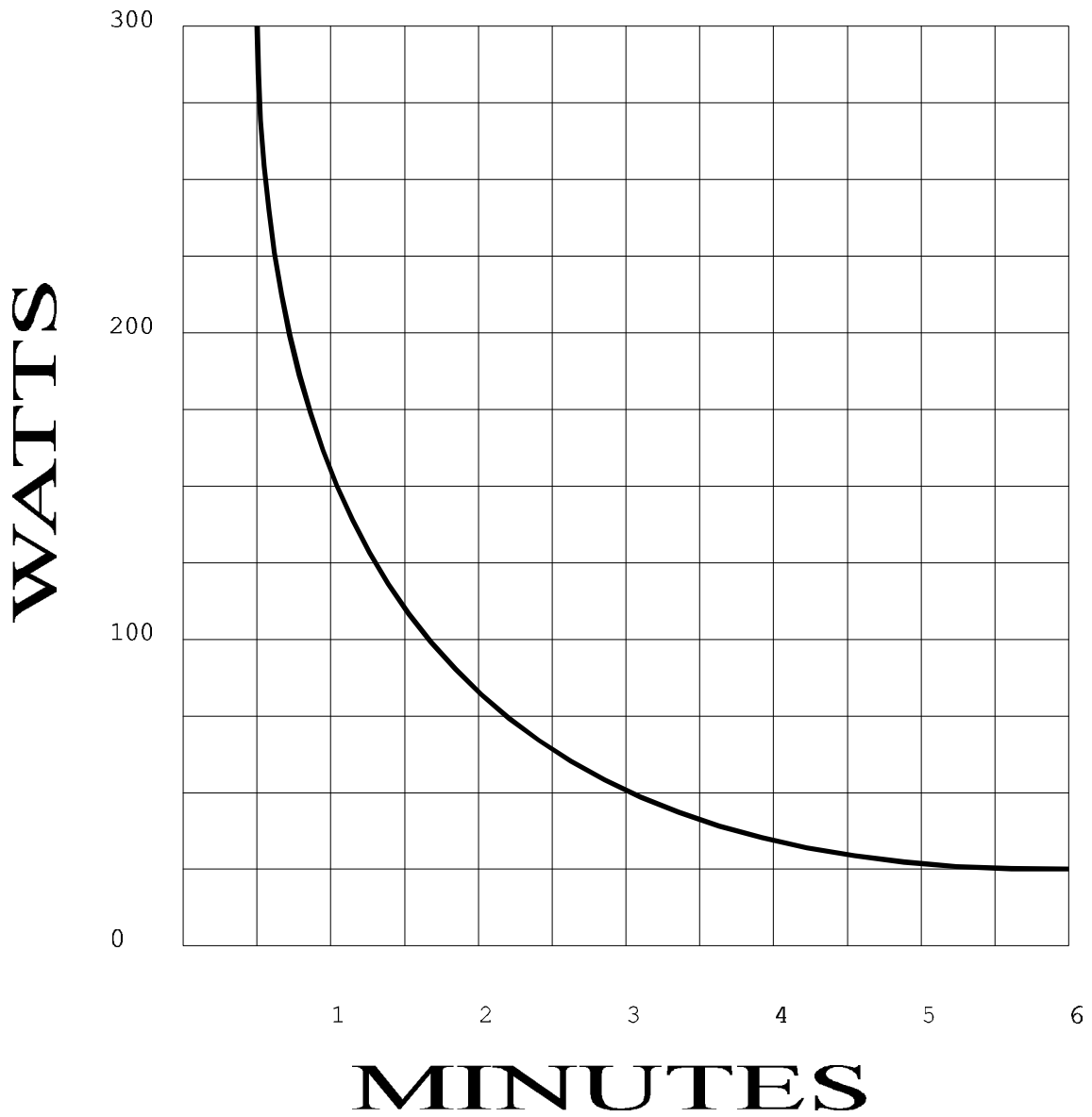
Derating curve for the MFJ260 Dummy Load.
